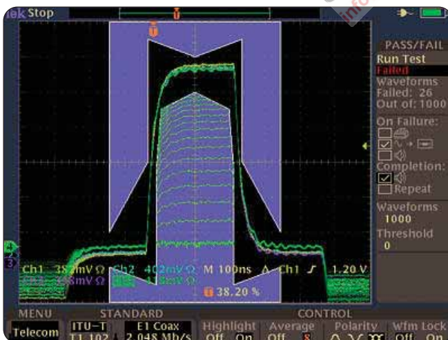
► The TDS3000C Series provides breakthrough test speeds for telecommunications line card testing. The telecom QUICKMENU puts all the commonly used telecom test functions on a single menu.
